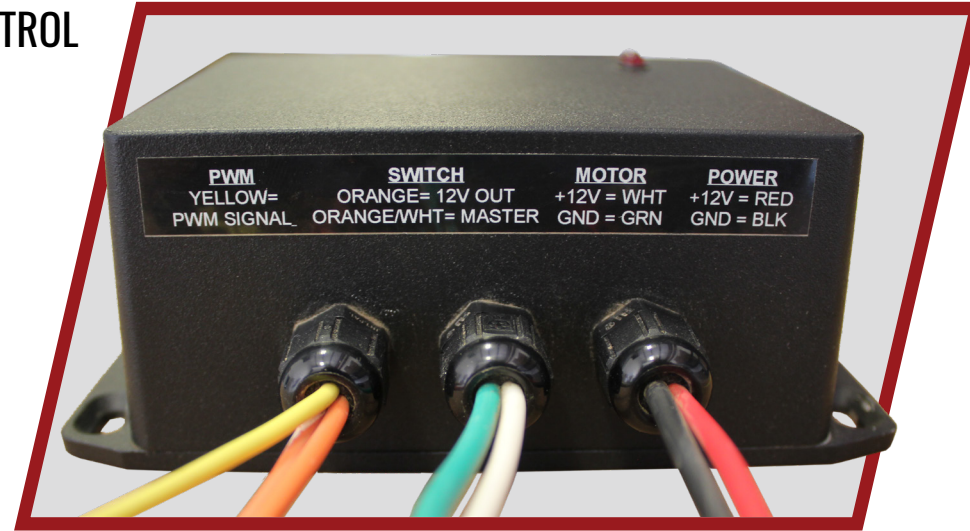
MSC-MOD PWM MOTOR CONTROLLER
